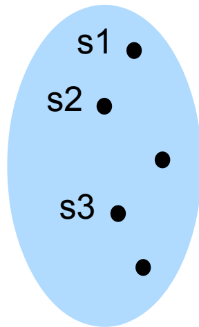
STUDENT
