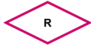
Relationship-Menge
