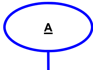
Schlüsselattribut
