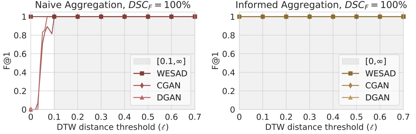
Figure 12: The "in-out" scenario on full overlap for Section 7.2. The x-axis gives the applied distance threshold and the y-axis shows the F@1 for our Slicing-DTW-Attack. We highlight the optimal threshold range across the tested datasets.
