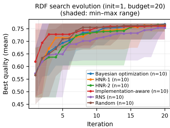
Figure 2: RDF pipeline search, best scores.
