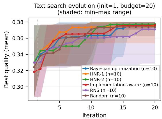
Figure 3: Text pipeline search, best scores.
