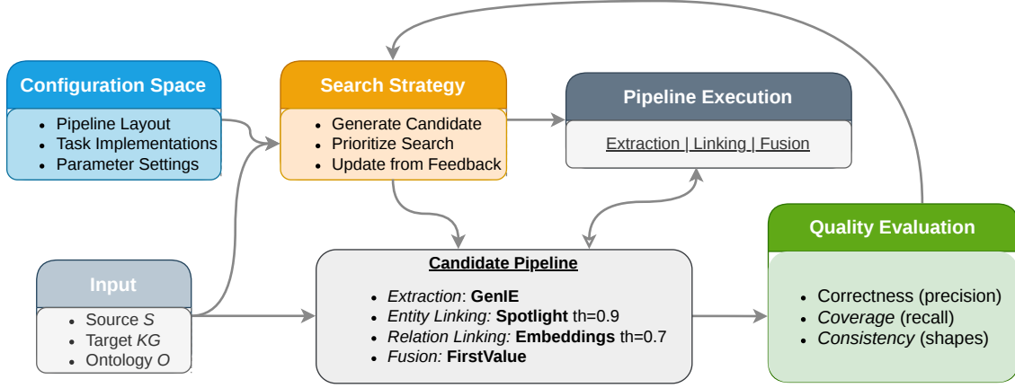
Figure 1: Overview of the quality-aware configuration search approach. The search strategy selects a valid pipeline configuration from the configuration space, instantiates and executes it on the input data, and uses the resulting knowledge graph quality as feedback for subsequent configuration choices. When the budget ( B ) is reached, it returns the best found pipeline of the search strategy.
